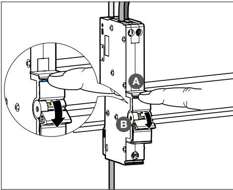
Fig 6: Testing the device ● Short press the test button T . The MCB-AFDD tripped, i.e. the circuit must switch off.
