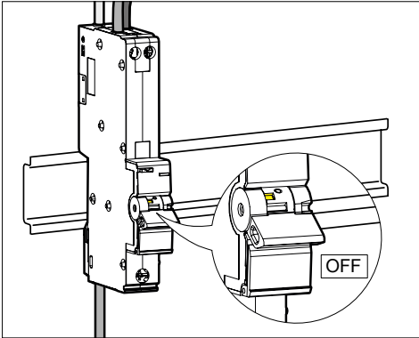
Fig 7: Handle position during testing: OFF The handle is in the OFF position. ● Keep the test button T pressed, to open the color code.
