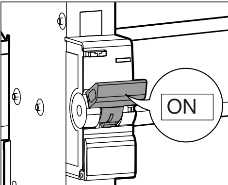
Fig 8: Handle during testing: ON The handle is in the ON position. ● Press the test button T for 5 seconds to activate bluetooth mode.
