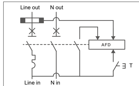
Fig 5: Wiring diagram
